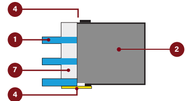
Panel with a thickness 2 mm in an INOX finish.
